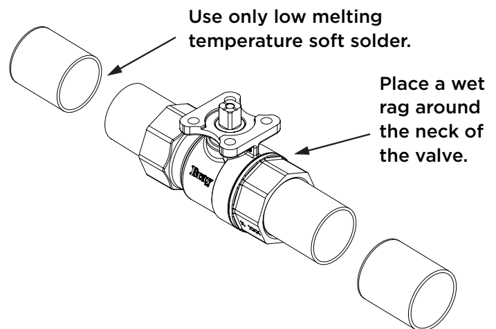
Figure 5: Sweat Valve Installation
