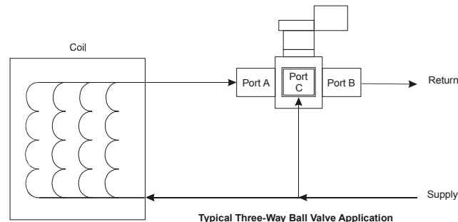
Typical Three-Way Ball Valve Application
