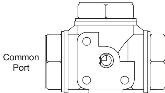
Figure 4: EBV Series Three-Way Ball Valve (Top View)
